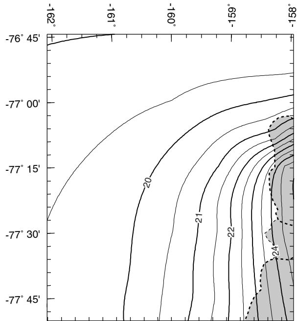
(e) Moho Model
