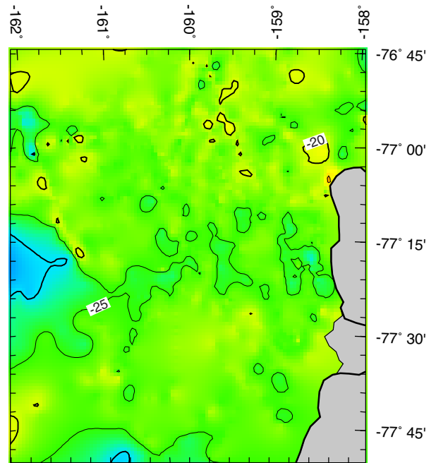
(f) FA Gravity Residual (5-Layer Model)
