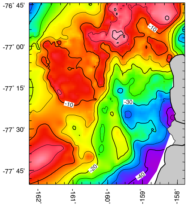
(c) FA Gravity Residual (3-Layer Model)
