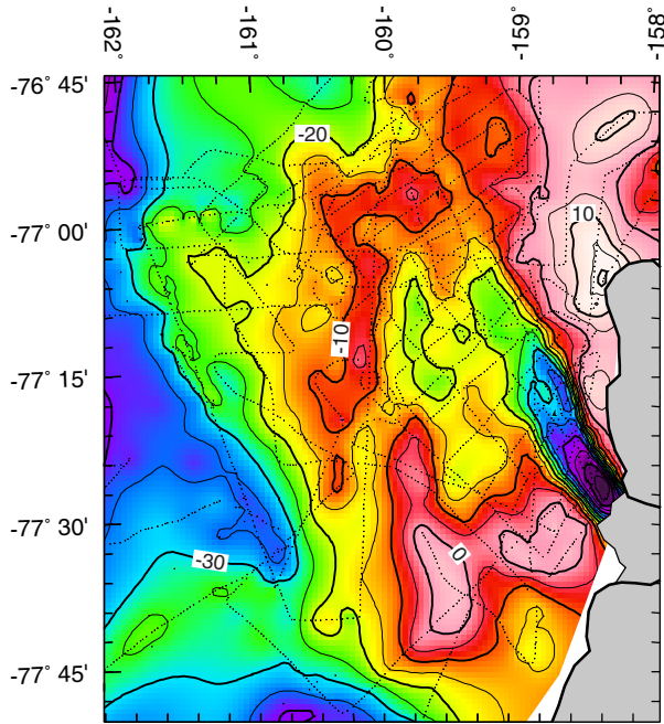
(a) Free Air Gravity Anomaly
