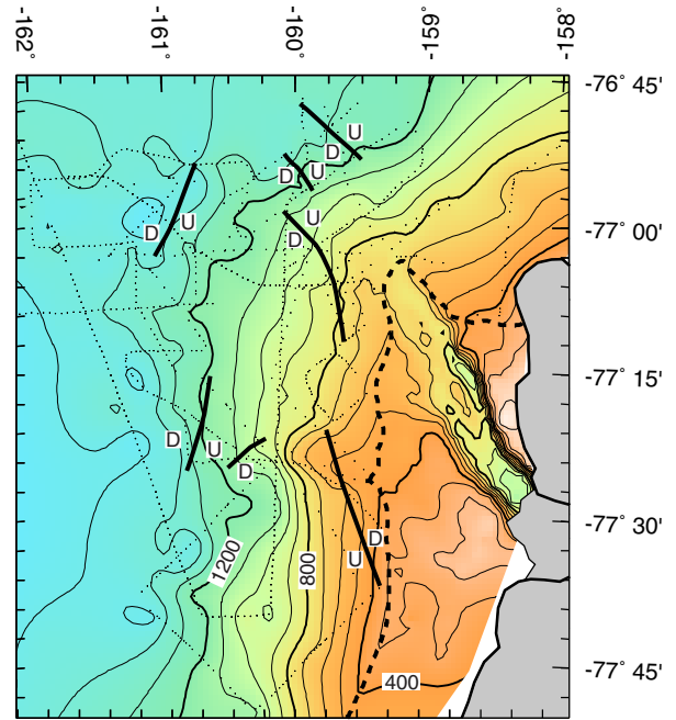
(b) Depth to Top RSS1 or Basement
